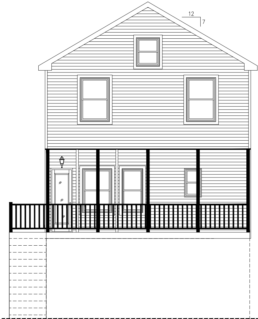
FRONT ELEVATION
