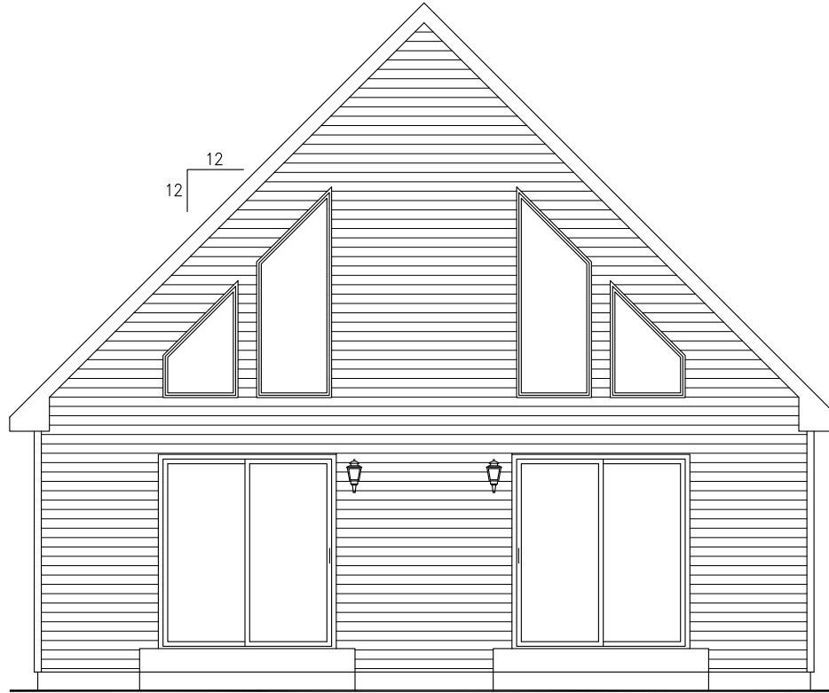
FRONT ELEVATION
