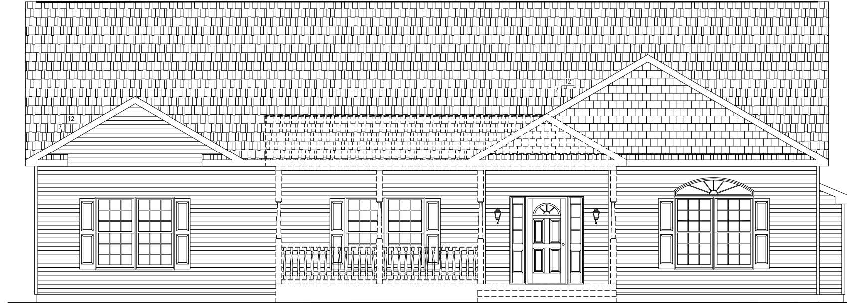
FRONT ELEVATION ACCESS TO GRADE ON-SITE BY OTHERS
