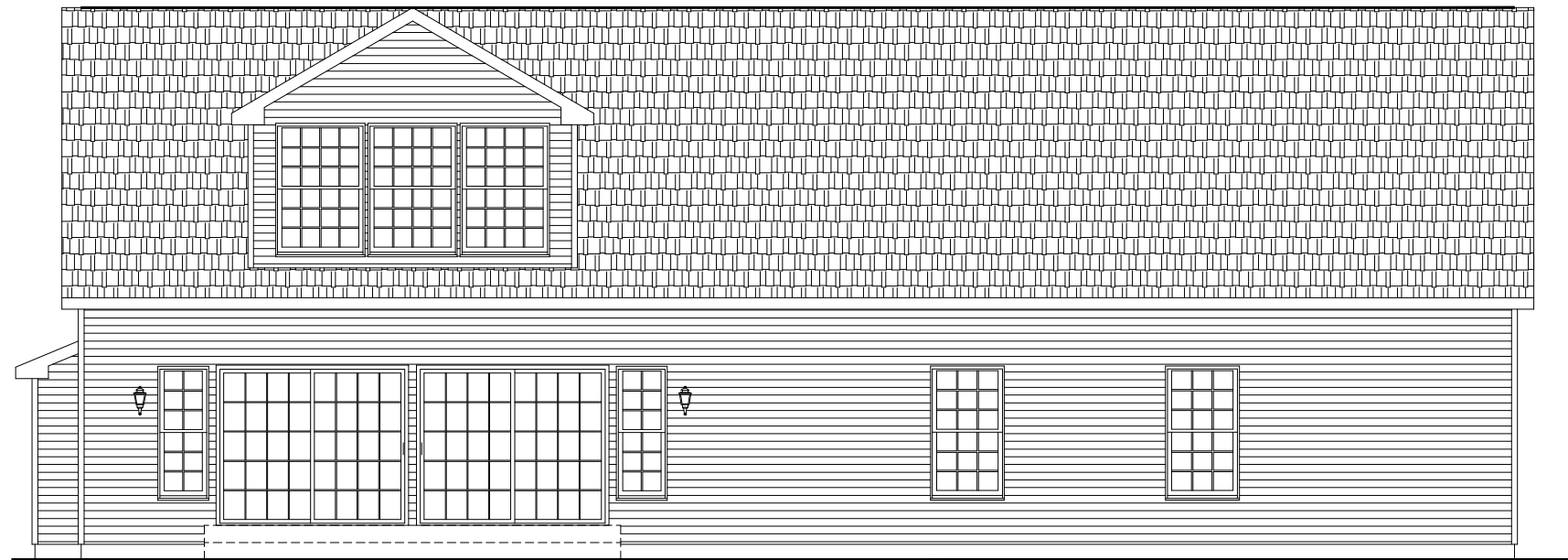
REAR ELEVATION ACCESS TO GRADE ON-SITE BY OTHERS
