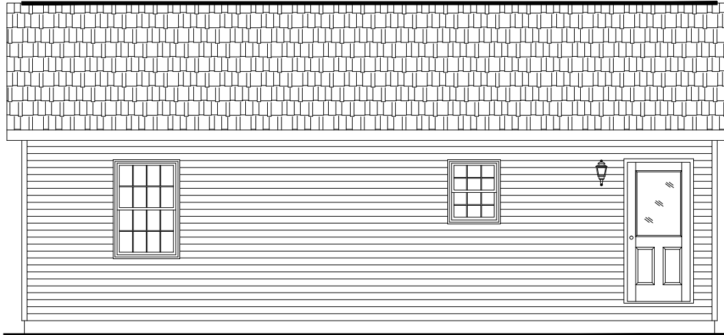
REAR ELEVATION
